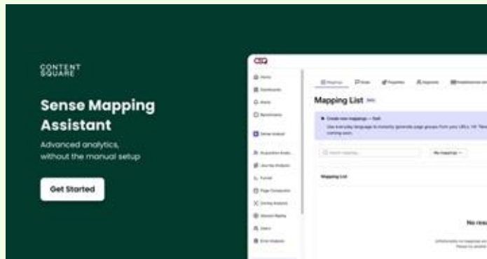
Sense for mappings
